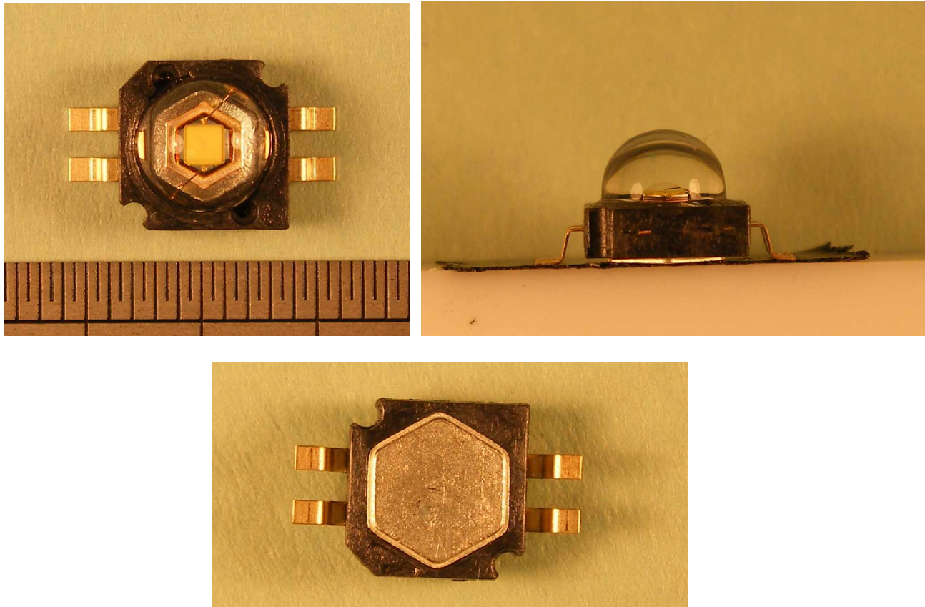
Figure 2.1 Top, side, and bottom views, with a scale in 0.5 mm increments. No branding or date code is seen on the device.
